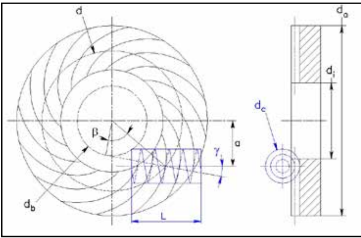
Figure 3: Schematics of right hand spiral face gear (black) hobbing with right hand hob (blue)
