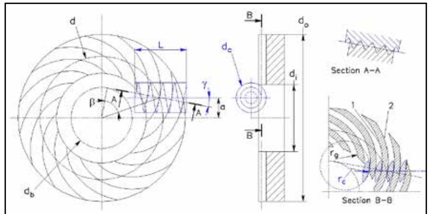
Figure 2: Schematics of left hand spiral face gear (black) hobbing with right hand hob (blue); \gamma – hob lead angle, L – hob length, d_c – hob major diameter; section A-A is tangent to base circle d_b and normal to the gear tooth line; section B-B is parallel to the hob axis, 1 – concave gear tooth flank, 2 – convex flank
