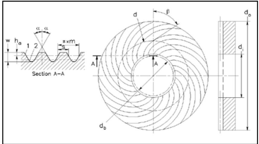
Figure 1: Face involute spiral gear; d_b , d_i , d , and d_o are base, minor, reference and major diameters, \beta is spiral angle at reference diameter, m – module, \alpha – profile (pressure) angle, s – tooth thickness at reference (pitch) line, w – whole depth; 1 – tooth flank, 2 – root fillet
