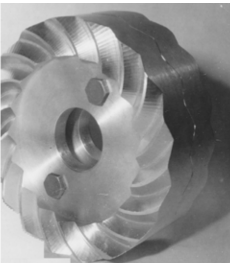
Figure 7: Sample of involute spiral face coupling assembly
