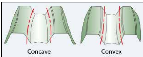
Figure 5: Curvic couplings
