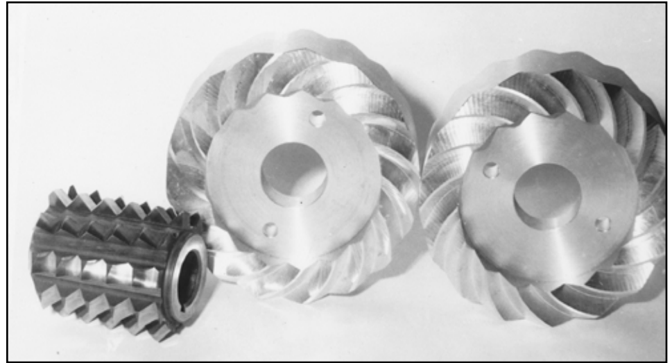
Figure 6: Experimental involute spiral face coupling mating flanges and hob (the same hob was used to machine both right and left hand spiral face gears)
