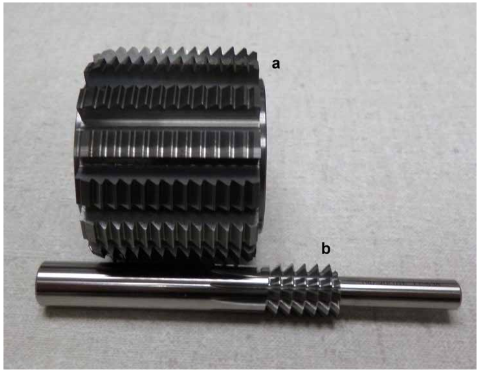
Figure 9: Asymmetric tooth hobs – a) helical pinion, b) spiral gear
